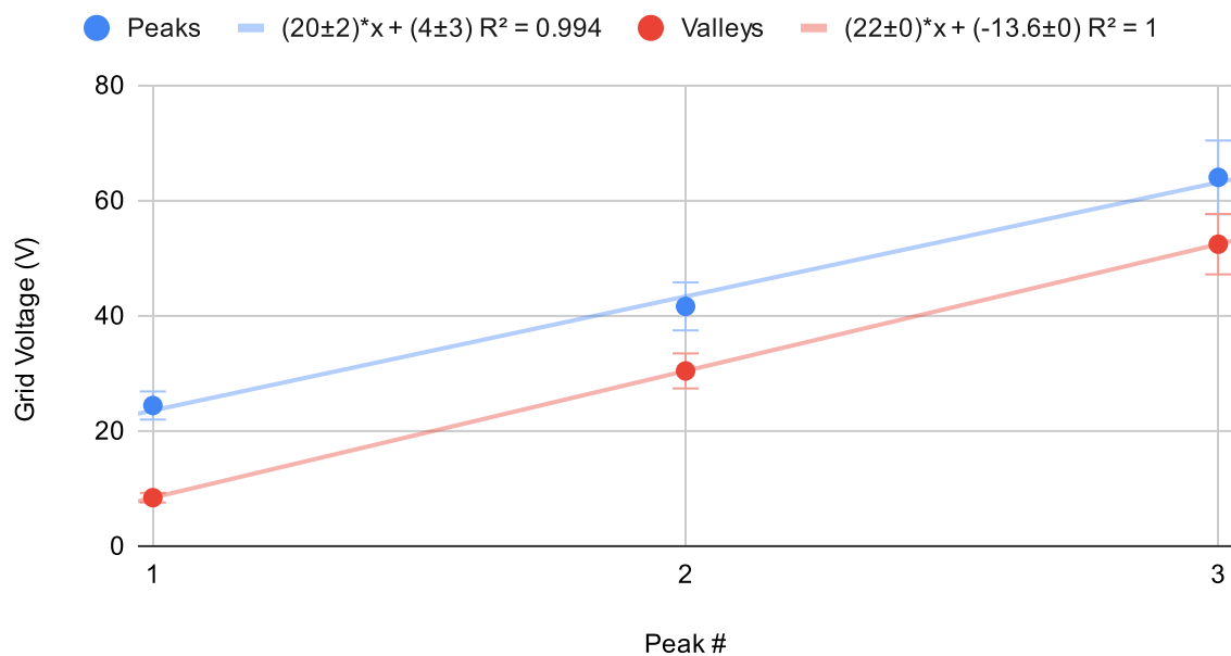
Figure 2: Grid Voltage ( V_G ) as a function of Peak Number. The solid line represents the linear best fit to the experimental data points. The equation of the fit and the R^2 value are as shown on the graph.
