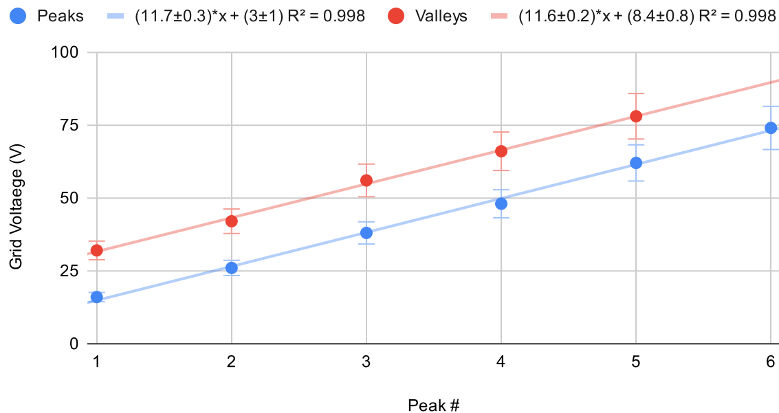
Figure 1: Grid Voltage ( V_G ) as a function of Peak Number. The solid line represents the linear best fit to the experimental data points. The equation of the fit and the R^2 value are as shown on the graph.
